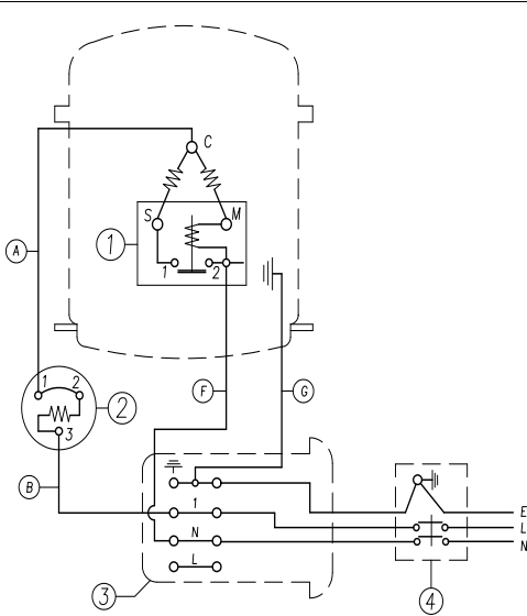
PUMP ELECTRICAL DIAGRAM
